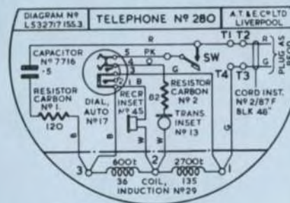
Wiring arrangements
