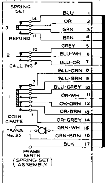
BOX, C.C. PART MECHANISM No. 7.
