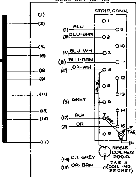
BELL SET No. 42.
