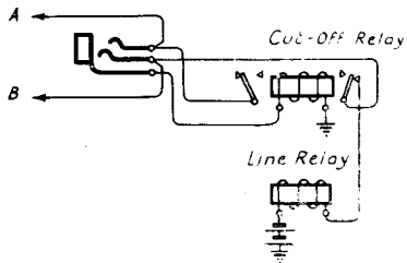
FIG. 3. LINE CIRCUIT, without Emergency Calling Facilities
