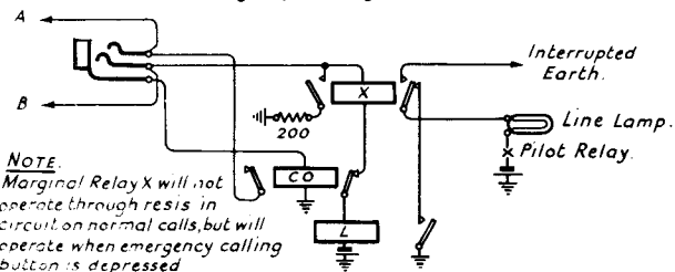
FIG. 4. LINE CIRCUIT, with Emergency Calling facilities.
