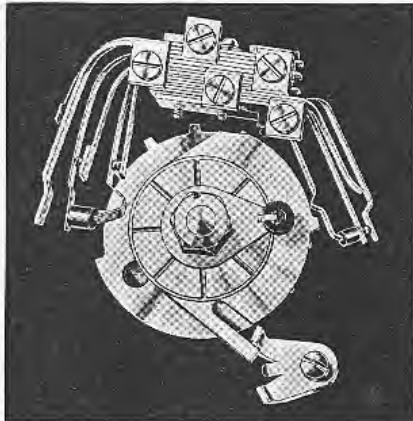
FIG. 5.—SLIPPING-CAM MECHANISM— DIAL WOUND-UP FOR DIGIT '5'
