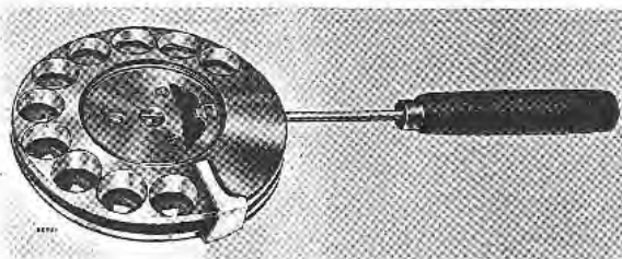
FIG. 19.—MOULDED BODY DIAL—REMOVAL OF LABEL PROTECTOR WITH SCREWDRIVER
