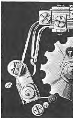
FIG. 11.—TRIGGER MECHANISM—TRIGGER MOVED AWAY FROM PULSE LEVER SPRING
