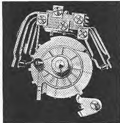
FIG. 4.—SLIPPING-CAM TYPE DIAL—MECHANISM NORMAL
