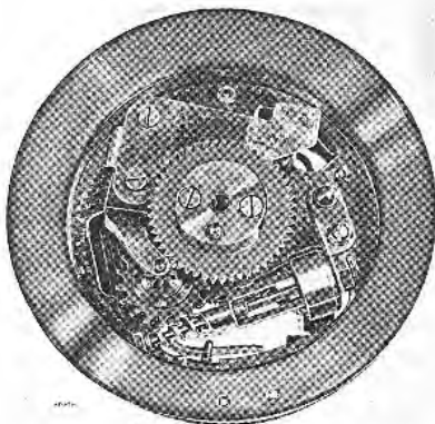
FIG. 9.—TRIGGER TYPE DIAL—GEAR TRAIN
