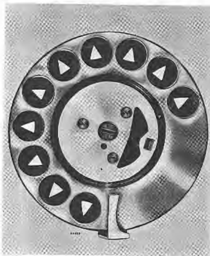
FIG. 15.—MOULDED BODY DIAL—FRONT VIEW
