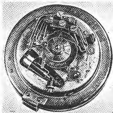
FIG. 2.—SLIPPING-CAM TYPE DIAL—REAR VIEW
