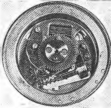
FIG. 3.—SLIPPING-CAM TYPE DIAL—GEAR TRAIN
