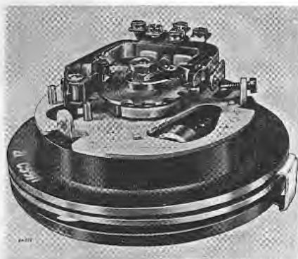
FIG. 16.—MOULDED BODY DIAL—REAR VIEW
