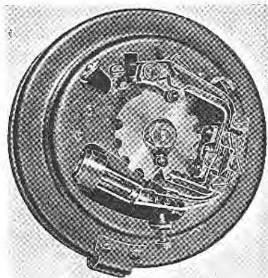
FIG. 8.—TRIGGER TYPE DIAL—REAR VIEW
