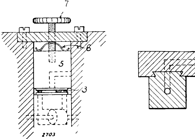
Fig. 19.—DETAILS OF AIR VALVE.
