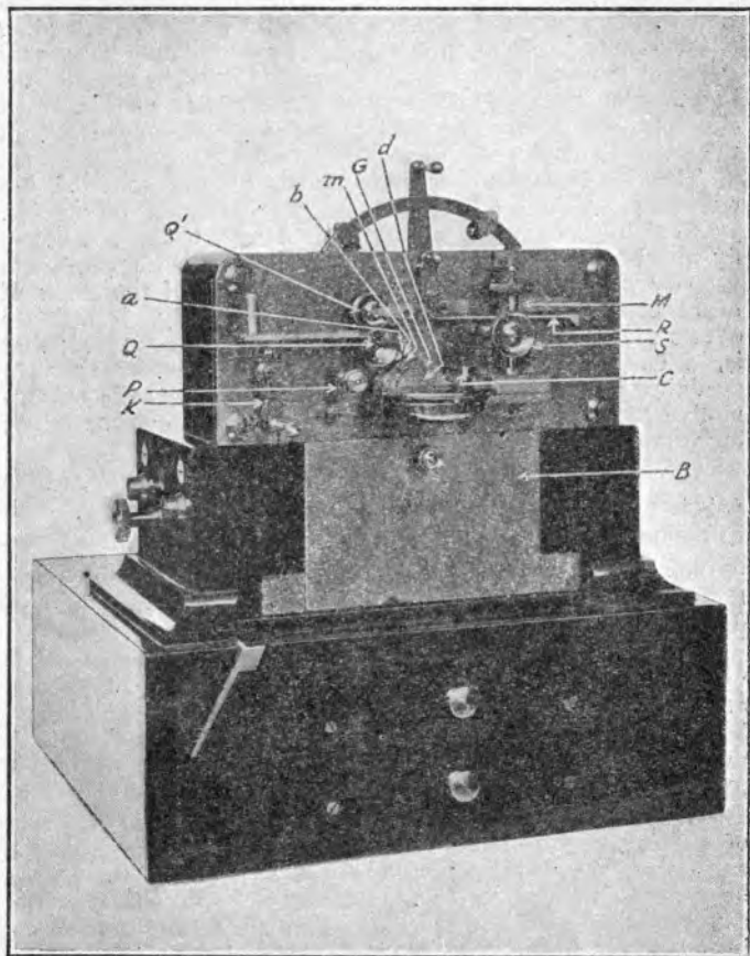
Fig. 7.—WHEATSTONE RECEIVER (LETTERED).
