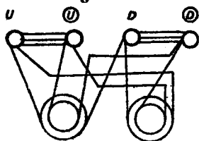
"COILS IN SERIES."
