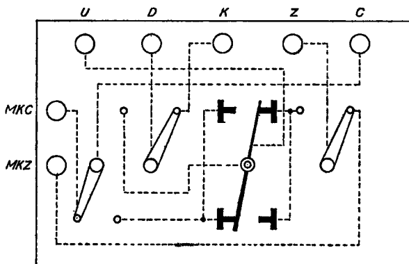
Fig. 4.—SWITCH CONNEXIONS OF WHEATSTONE TRANSMITTER.
