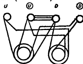
"COILS IN PARALLEL."
