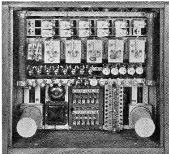
FIG. 20.—SWITCHBOARD TELEPRINTER NO. 18. REAR VIEW.
