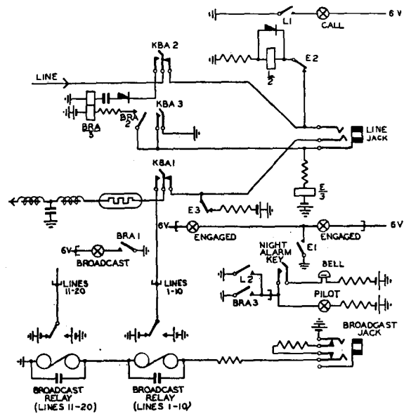
FIG. 8.—TELEPRINTER SWITCHBOARD. LINE TERMINATION WITH BROADCASTING FACILITIES.
