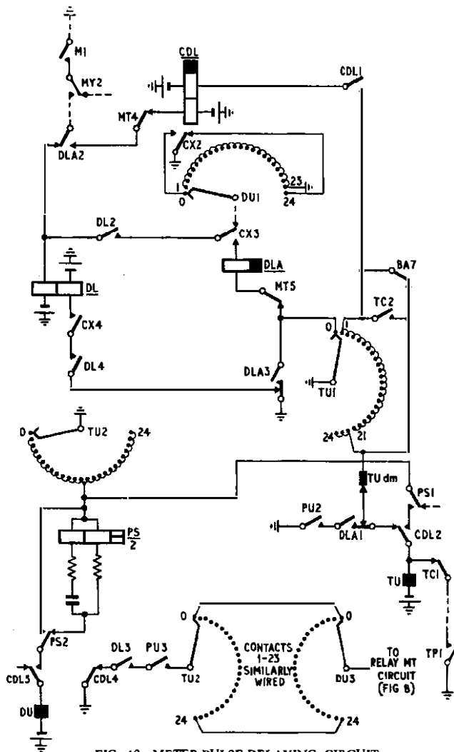
FIG. 10—METER-PULSE-DELAYING CIRCUIT
