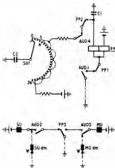
FIG. 13—AUDIT CIRCUIT
