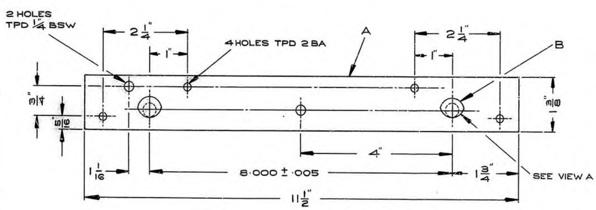
15/60577 MATERIAL: REFA STEEL CR HH 4GP BS1449 (6.35 mm) REF B STEEL 240M07 BS 970
