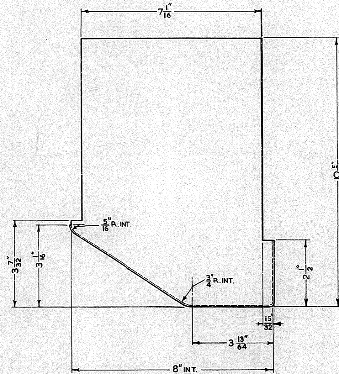
SHELF No. 2 MATERIAL FINISH } SEE SPEC.
