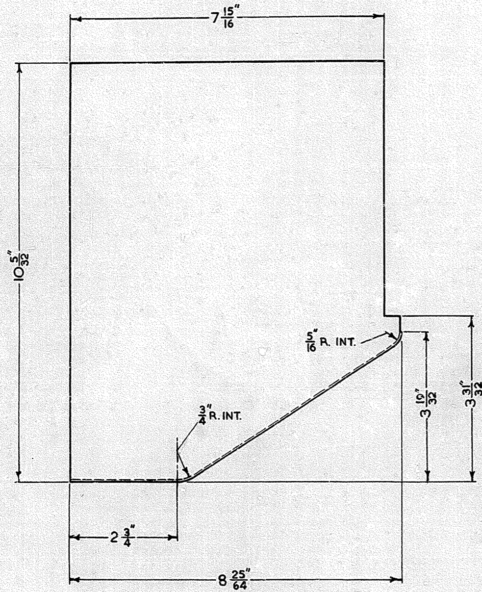
SHELF No. 1 MATERIAL FINISH } SEE SPEC.
