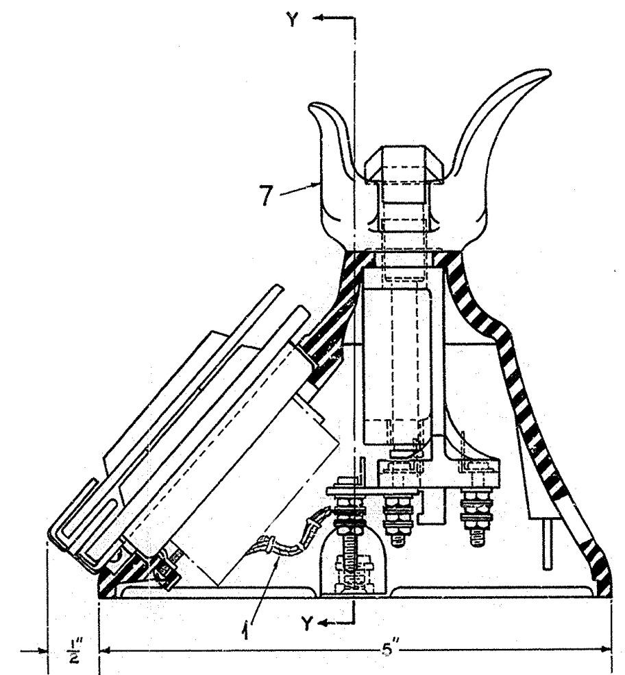
PART SECTION X - X (ITEM 5 OMITTED)
