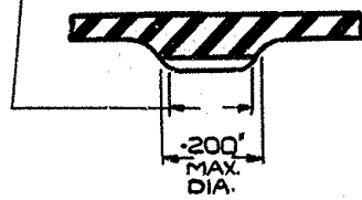
ENLARGED SECTION ON B-B SCALE: - 4/1
