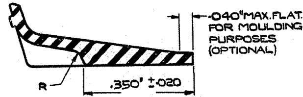
ENLARGED SECTION ON C-C SHOWING DETAILS OF RECESS SCALE: - 4/1
