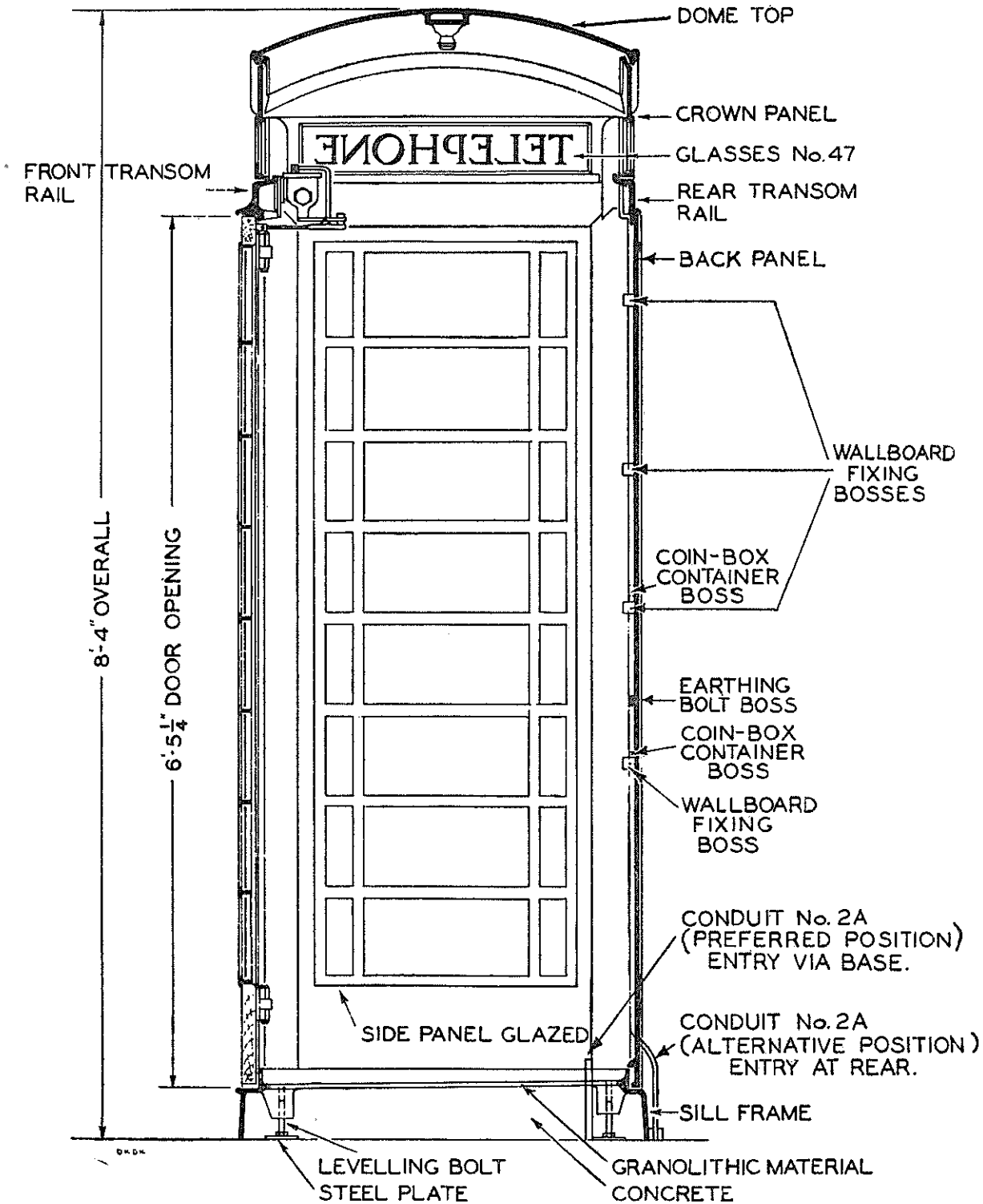
FIG. 1. KIOSK No. 6—SHOWING COMPONENT PARTS
