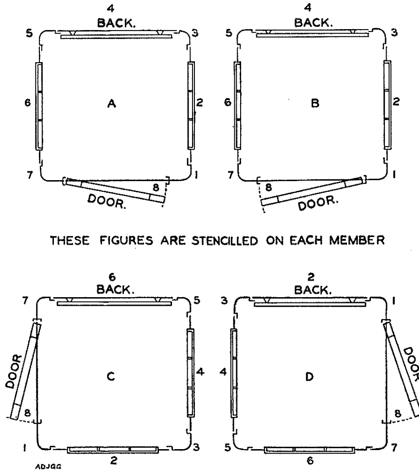
FIG. 2. KIOSK NO. 6—NUMBERING OF SECTIONS AND IDENTIFICATION OF ASSEMBLIES
