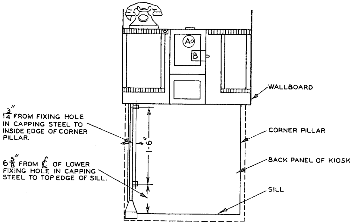
FIG. 3B. POSITION OF CAPPING, STEEL NO. 6 ON BACK PANEL
