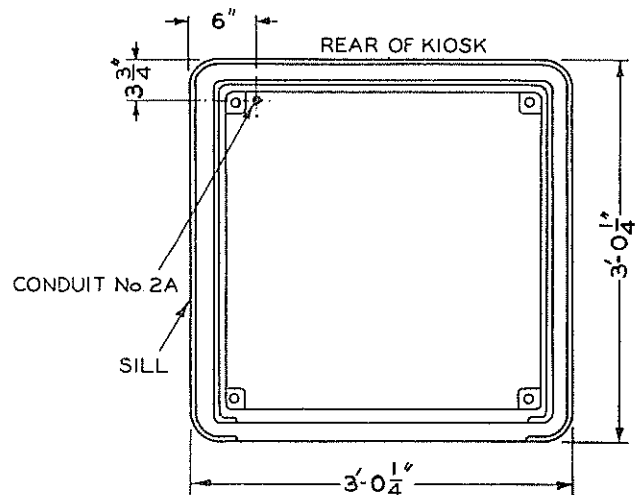
FIG. 3A. POSITION FOR LEAD-IN CONDUIT NO. 2A, WHEN CAPPING, STEEL, NO. 6 IS USED
