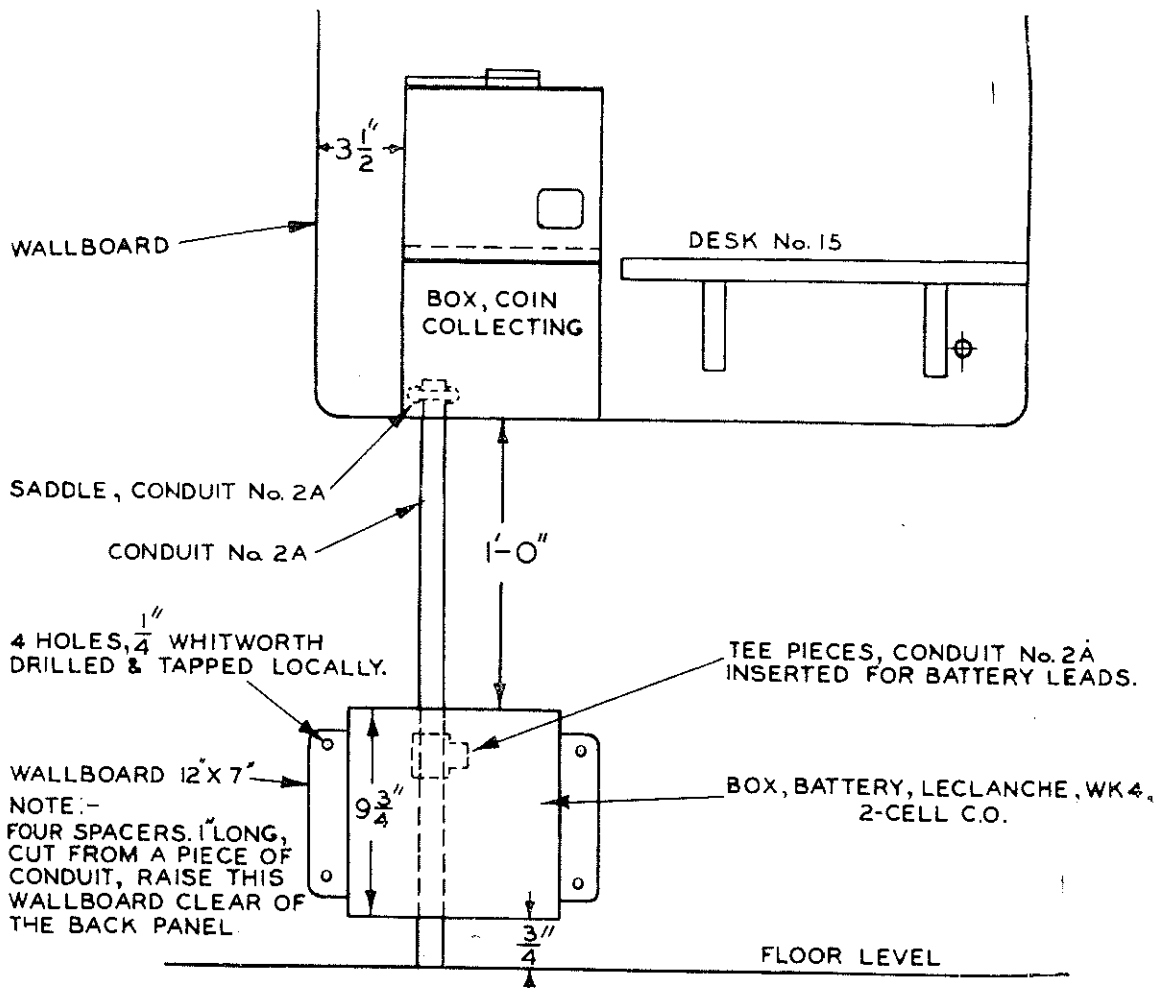
FIG. 4. KIOSKS IN MAGNETO AREAS—LEAD-IN ARRANGEMENTS
