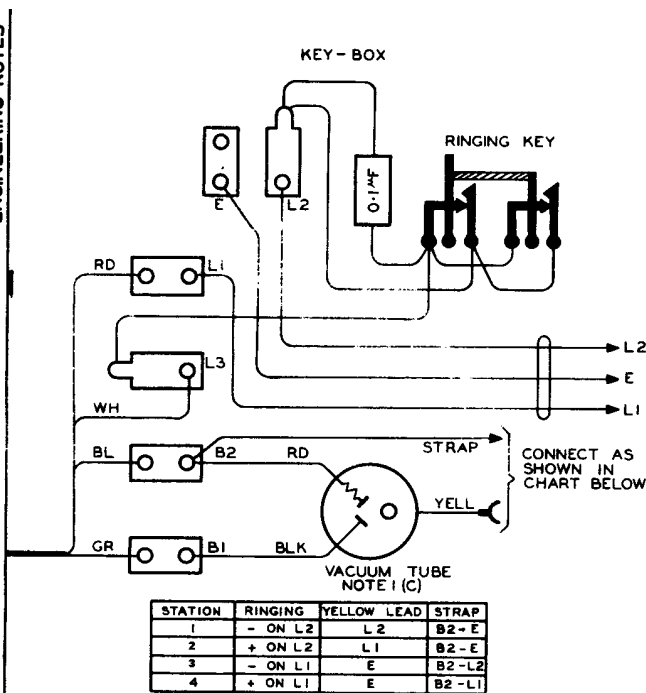
FIG. 1 WIRING OF EXTN. TELEPHONE (RINGING) TO MAIN. NOTE 4
