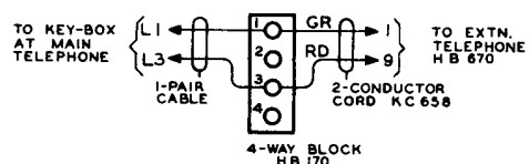
FIG. 2 WIRING OF EXTN. TELEPHONE (NON-RINGING) TO MAIN. NOTE 5
