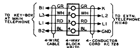
FIG. 1 WIRING OF EXTN. TELEPHONE (RINGING) TO MAIN. NOTE 4
